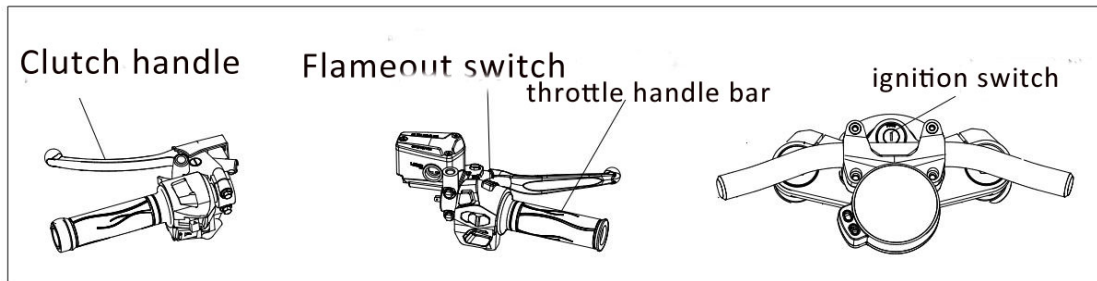
Fig 11 Start preparation
